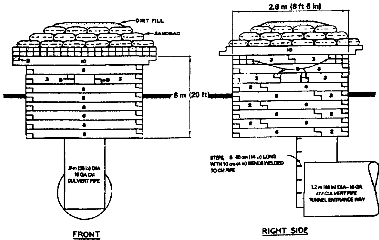
Figure 1-55. Concrete log bunker.
